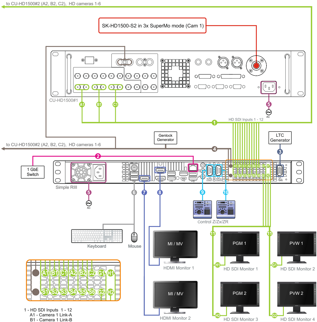
Connection diagram
